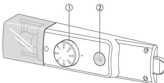
(1) Temperature controller
